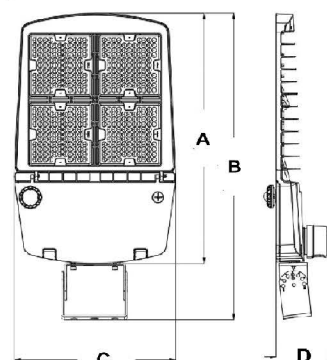
Trunnion mount A. 19 1/4" B. 22 1/8" C. 10 7/16" D. 3 1/4"
