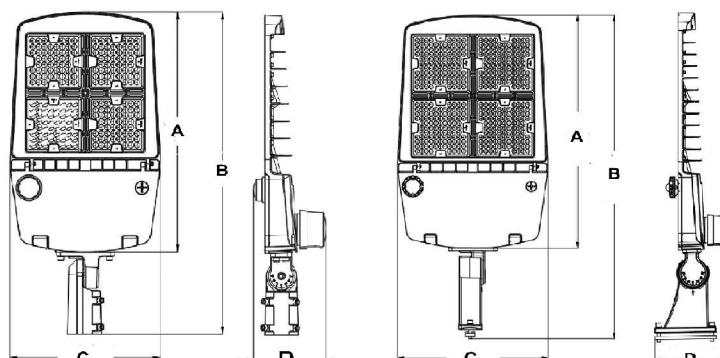
Direct mount A. 19 1/4" B. 23 3/4" C. 10 7/16" D. 6 3/16"
