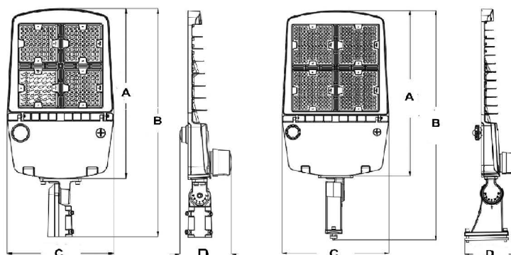
Direct mount
